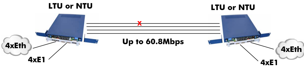
Point-to-Point Bonding Application with Failure Protection
